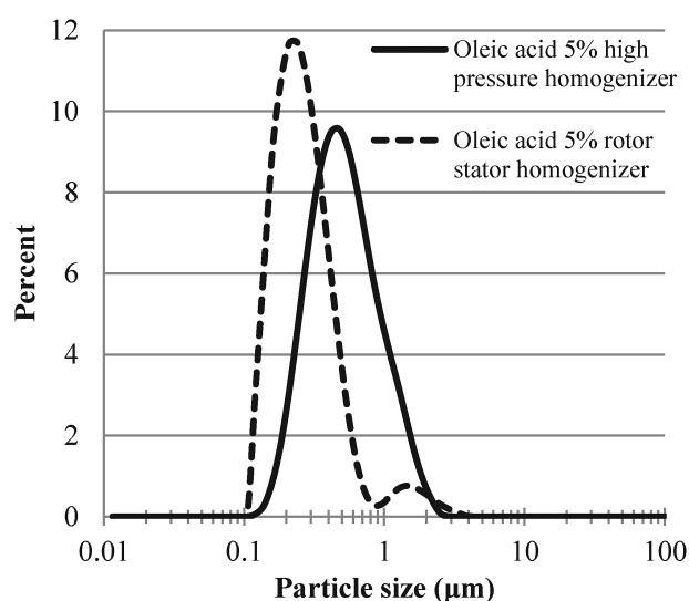
Figure 2. Particle sizes of highest concentration emulsions.
