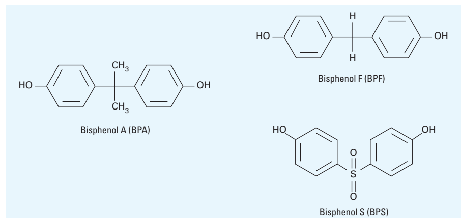
Figure 1. Chemical structures of bisphenol A, bisphenol S, and bisphenol F.
