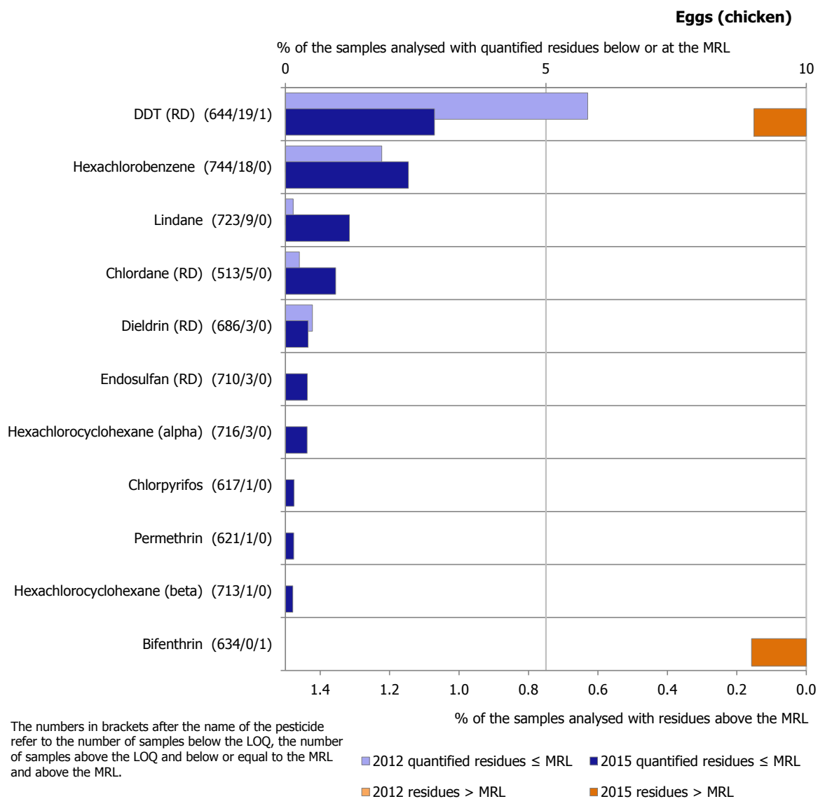
Figure 33: Percentage of chicken eggs samples with quantified residues below or equal to the MRL
