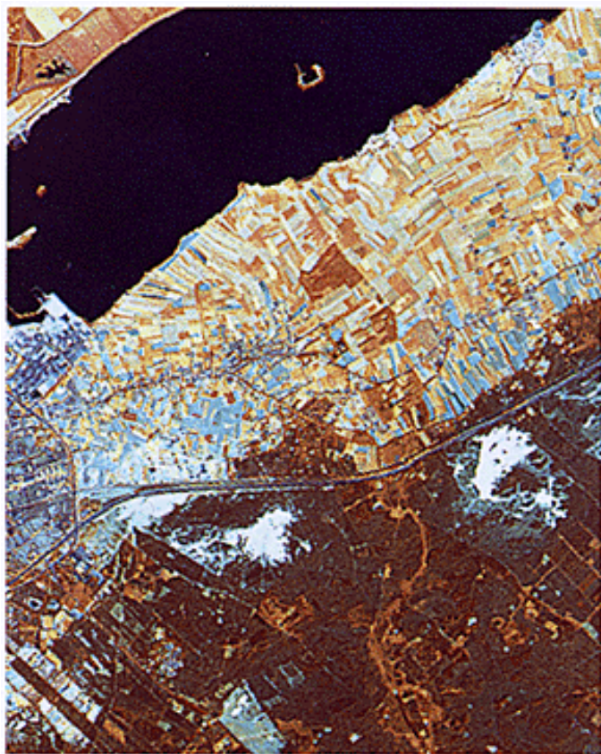
3.1.2. Netherlands/Area: Hardewijk Landsat TM 4.5.3. 1:100 000, May 1989
