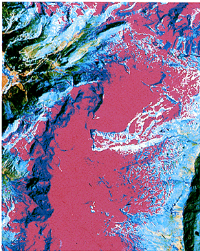
3.3.5. France/Area: Vanoise Landsat TM 4.5.3. 1:100 000, June 1991
