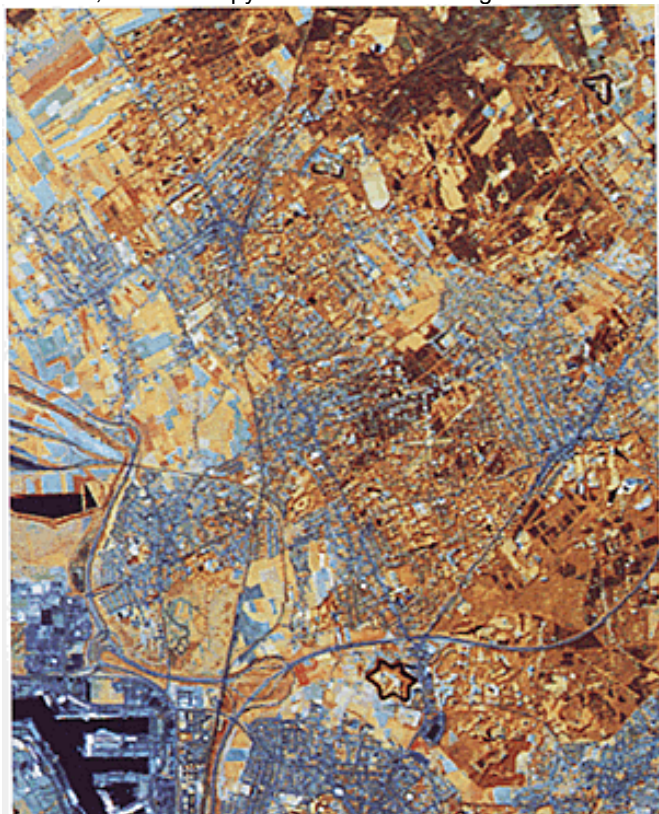
Belgium/Area: Brasschaat Landsat TM 4.5.3 1:100 000, May 1989
