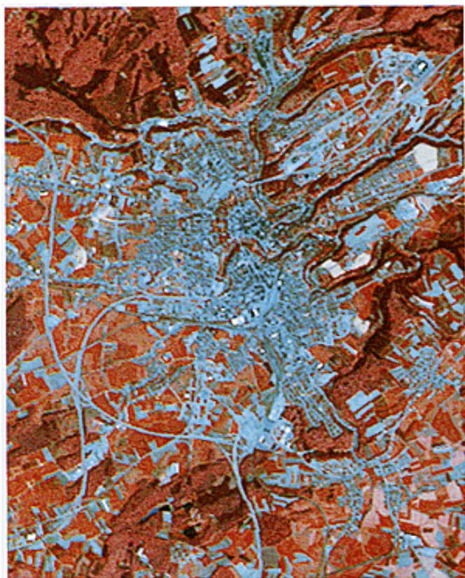
1.1.1. Luxembourg/Area: Luxembourg City Landsat TM 4.3.2. 1:100 000, August 1989
