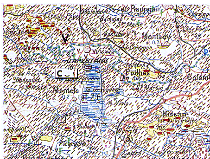
Vegetation map (scale 1:200 000)
