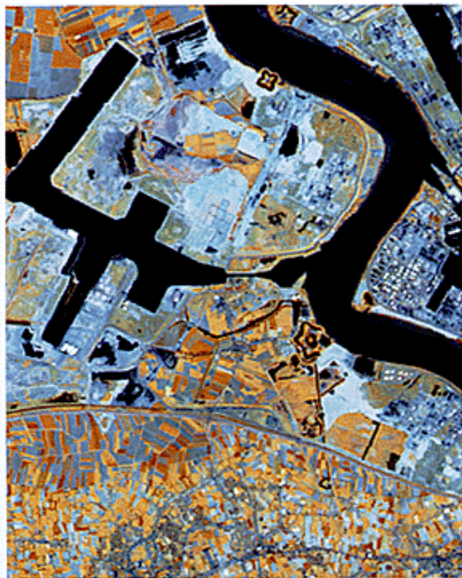
1.3.3. Belgium/Area: Antwerp Landsat TM 4.5.3. 1:100 000, May 1989
