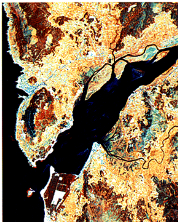
Portugal/Area: Caminha Landsat TM 4.5.3. 1:100 000, July 1987
