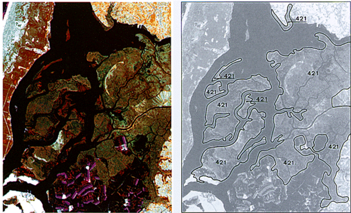
4.1.2. Ireland/Area: Rathagan Landsat TM 4.5.3. 1:100 000, May 1990
