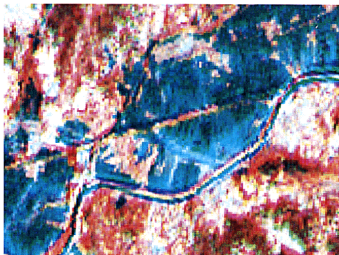
Landsat MSS 7.5.4 (scale 1:100 000, May 1986)
