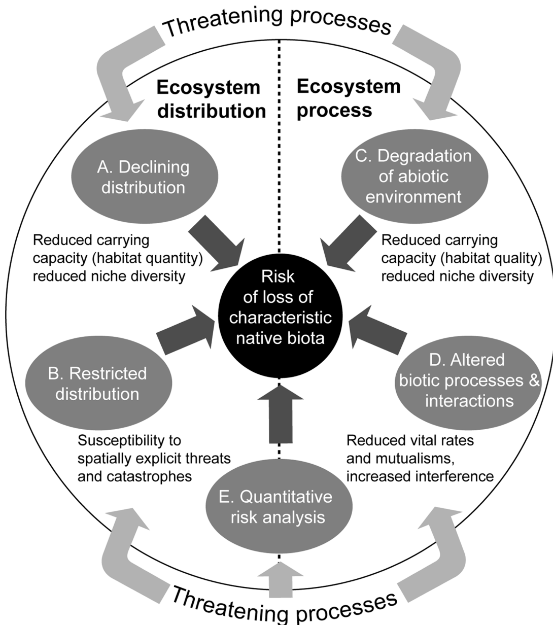
Figure 2. Mechanisms of ecosystem collapse, and symptoms of collapse risk.
