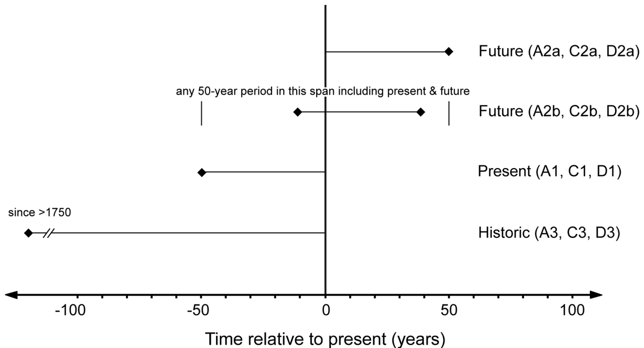
Figure 4. Time scales for assessment of change under criteria A, C and D.
